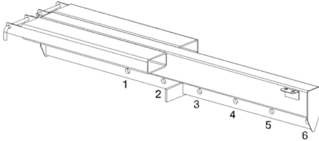
Position of the safety lifting hook
