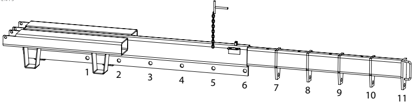
Position of the safety lifting hook
